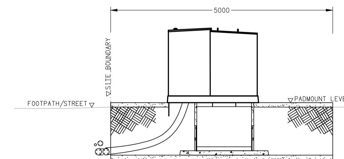
DETAIL A PADMOUNT SECTION VIEW SCALE 1:50
